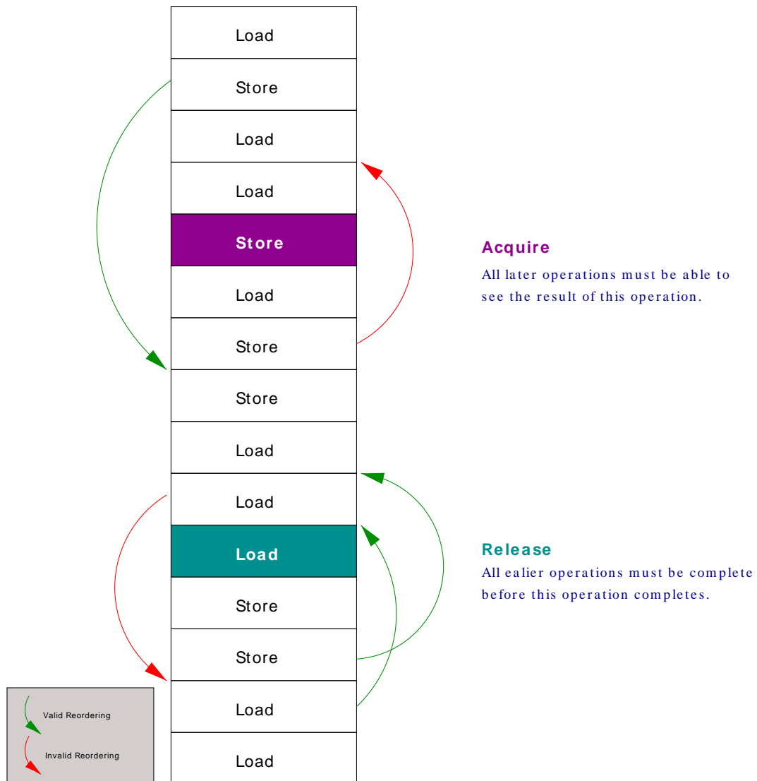
Figure 3.9. Acquire and Release semantics
