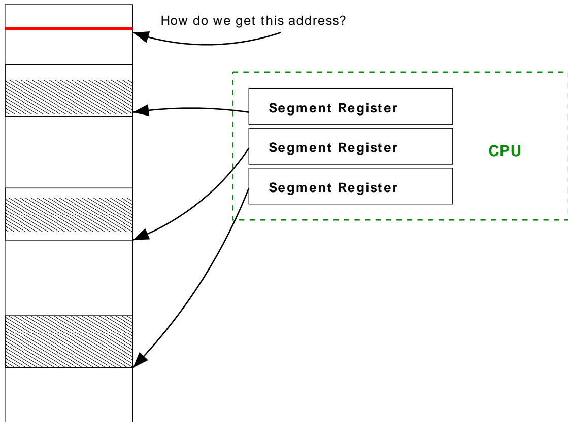
Figure 6.4. Segmentation
