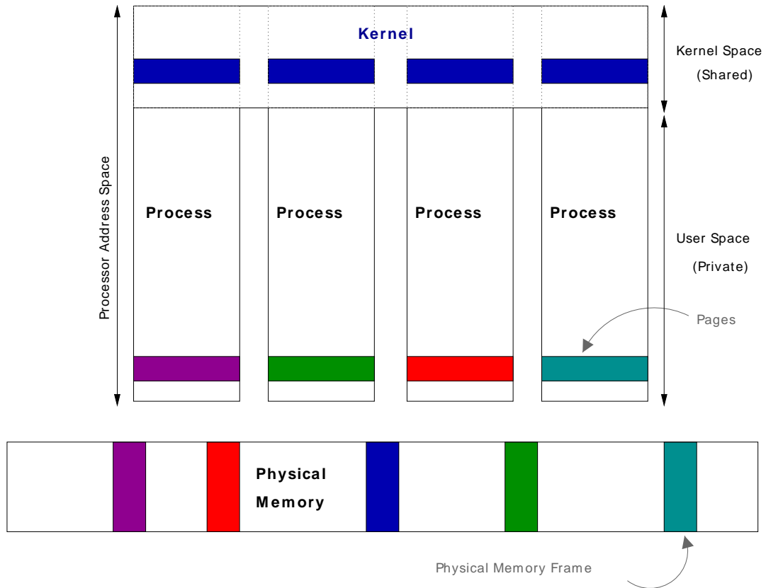
Figure 6.5. Linux address space layout
