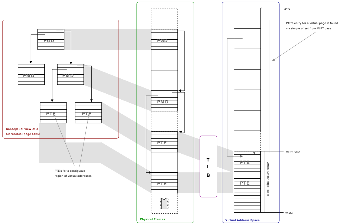
Figure 6.10. Itanium short-format VHPT implementation
