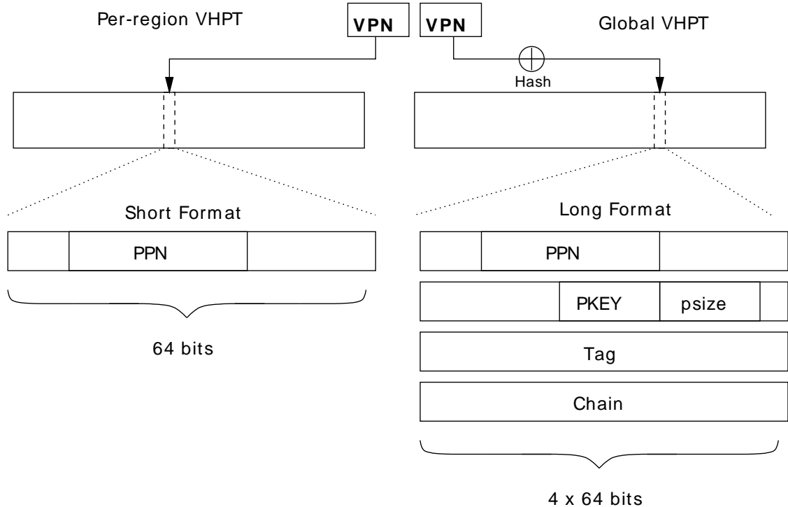
Figure 6.11. Itanium PTE entry formats
