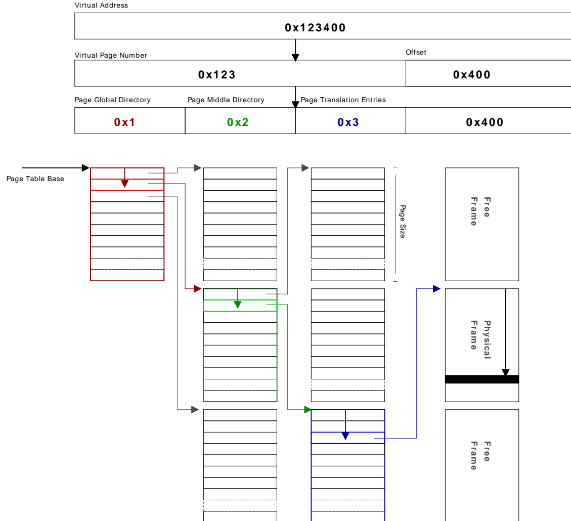
Figure 6.9. Illustration of a hierarchical page-table
