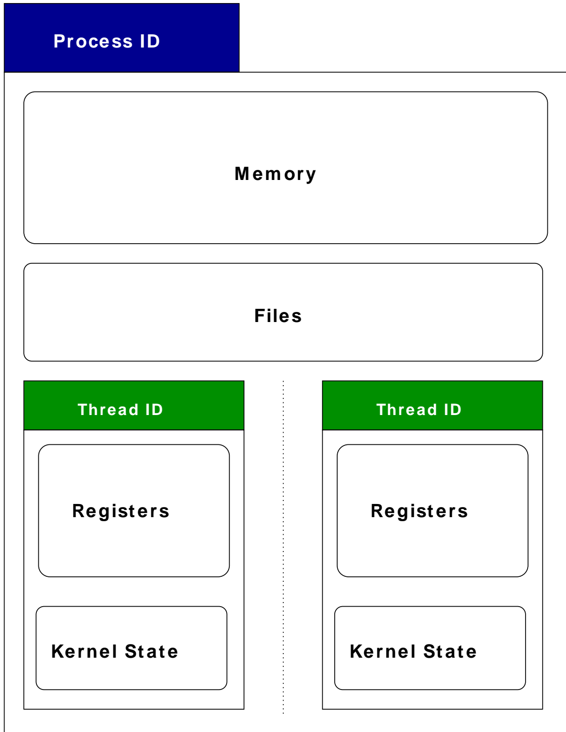
Figure 5.4. Threads
