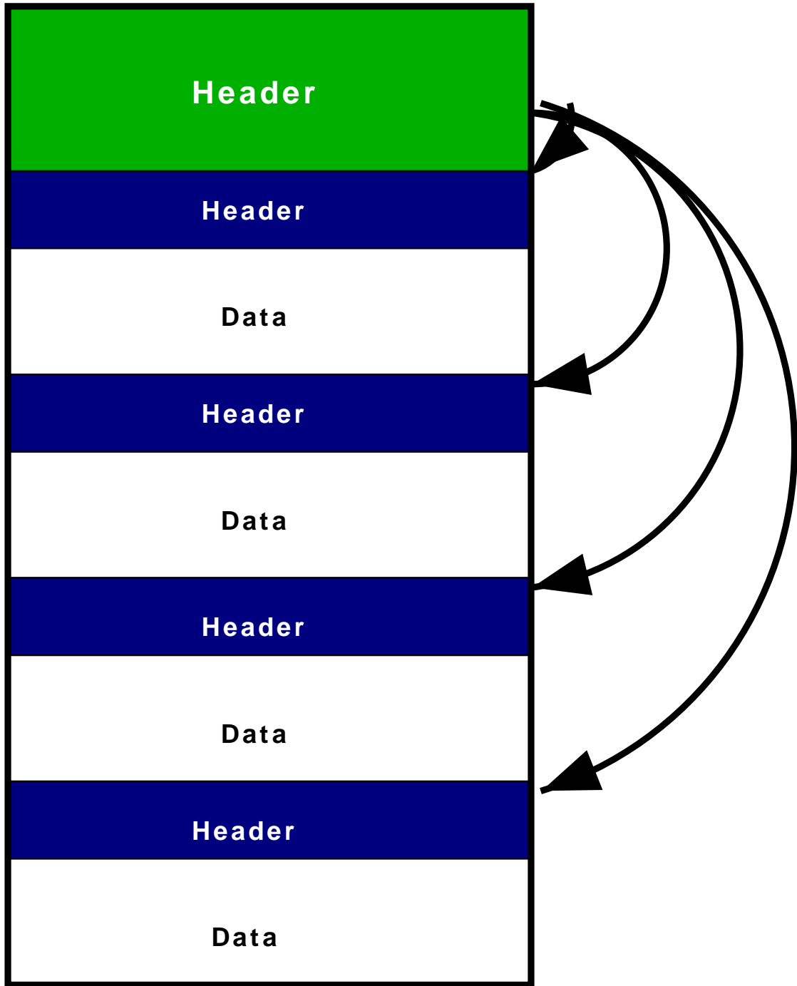
Figure 8.1. ELF Overview
