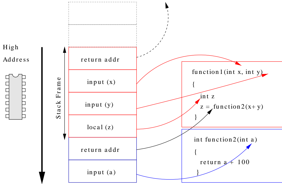
Figure 5.2. The Stack
