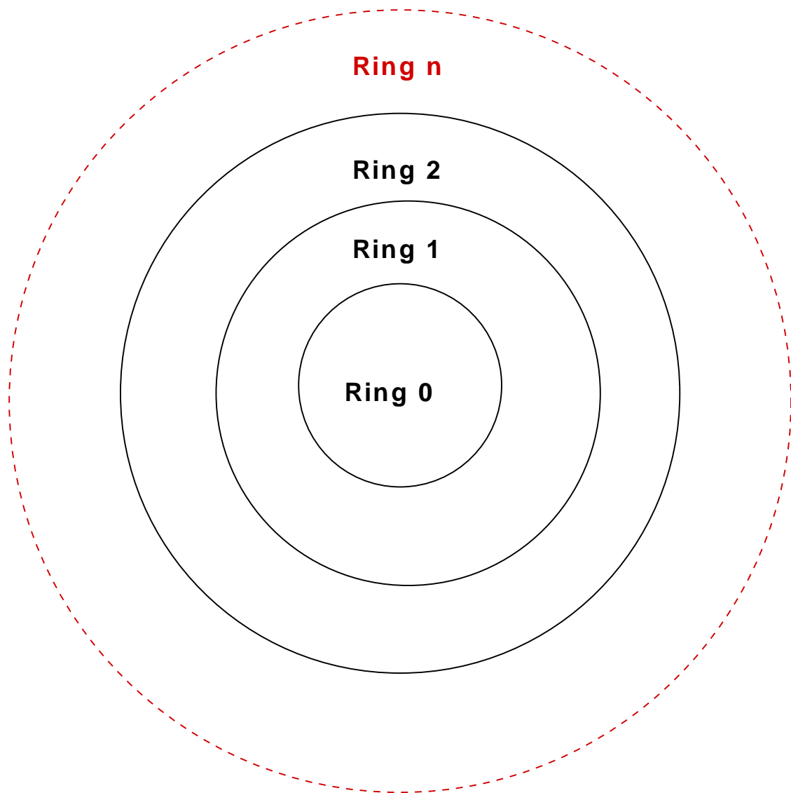
Figure 4.3. Rings
