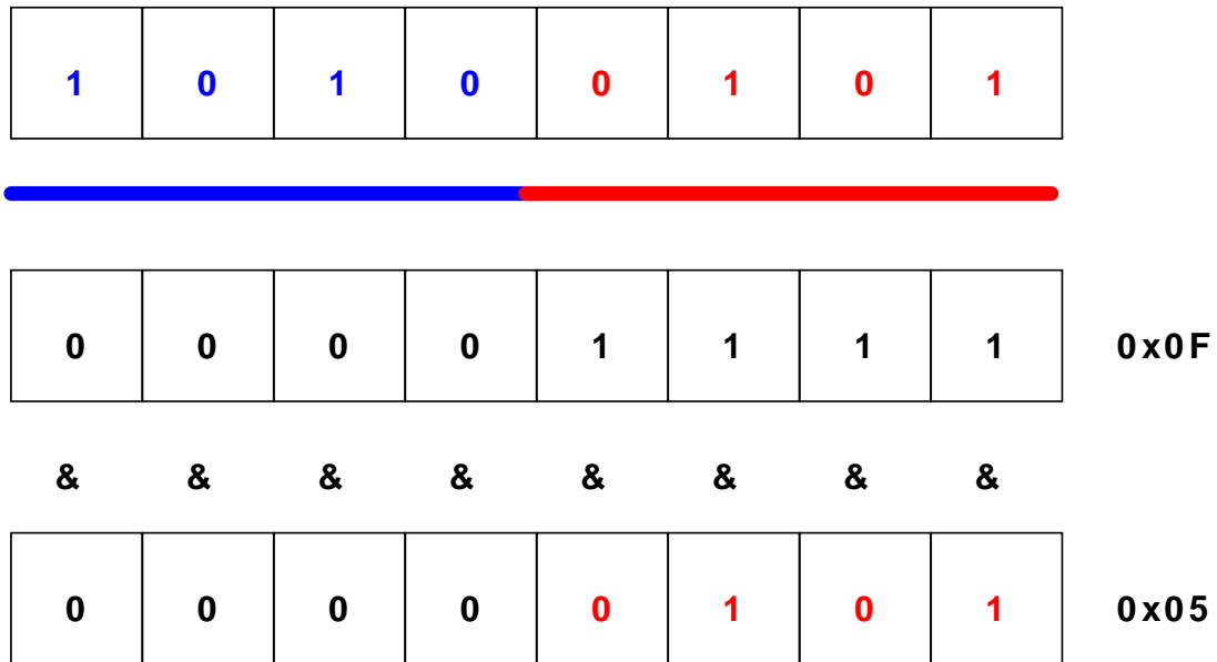
Figure 2.1. Masking
