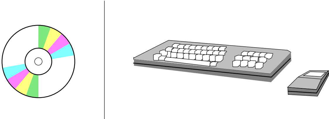
Figure 1.1. Abstraction
