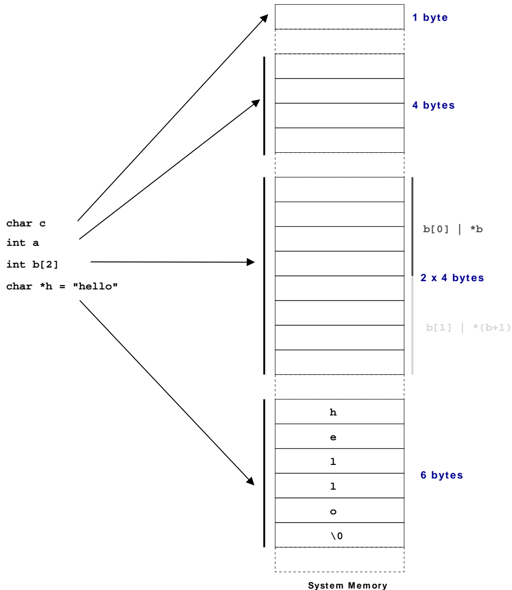
Figure 2.2. Types
