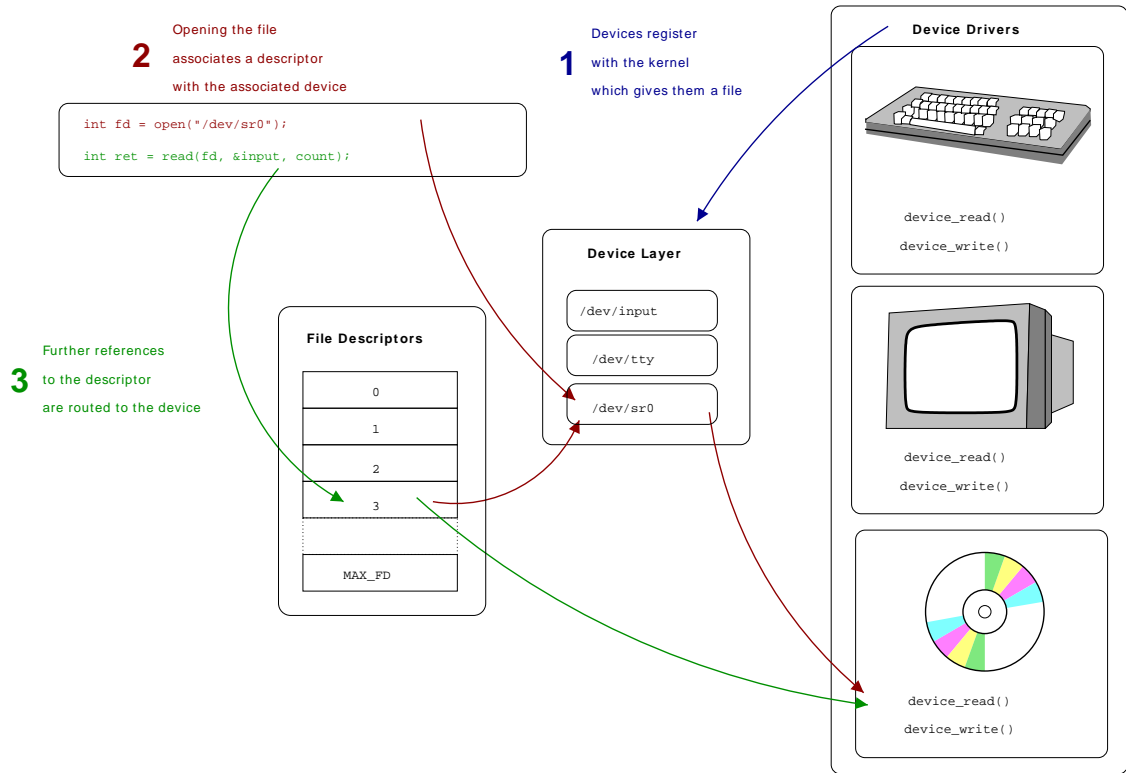
Figure 1.3. Abstraction
