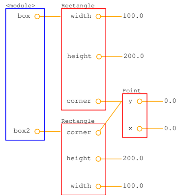
Figure C.5: Object diagram.
